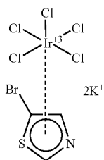
K_2[IrCl_5(5\text{-bromo-thiazole})]
